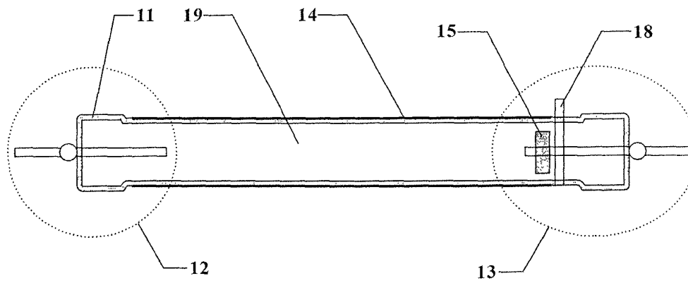
Fig. 1: Side Elevation of current Flash discharge Lamp.
