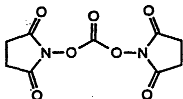
di(N-succinimidyl) carbonate
