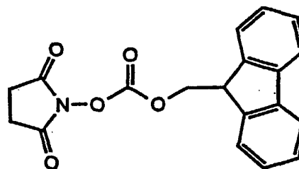
N-(9-fluorenylmethoxycarbonyloxy)succinimide
