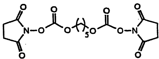
1,5-bis(succinimidooxycarbonyloxy)pentane
