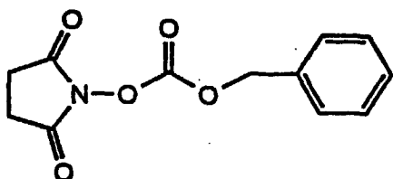
N-(benzyloxycarbonyloxy)succinimide
