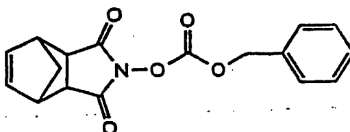
N-benzyloxycarbonyloxy-5-norbornene-2,3-dicarboximide
