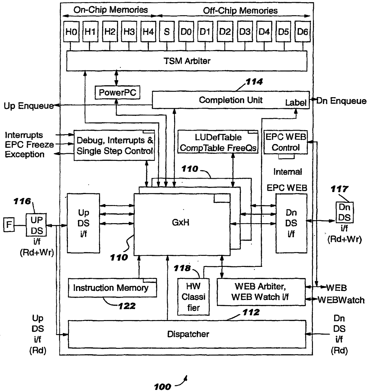
FIG. 2 BLOCK DIAGRAM OF THE EPC
