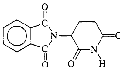
thalidomide
