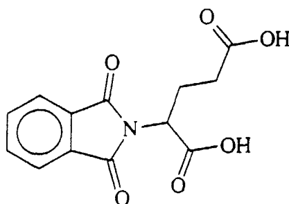
phthaloyl glutamic acid (PG Acid)
