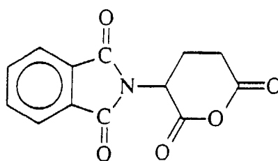
phthaloyl glutamic anhydride (PGA)
