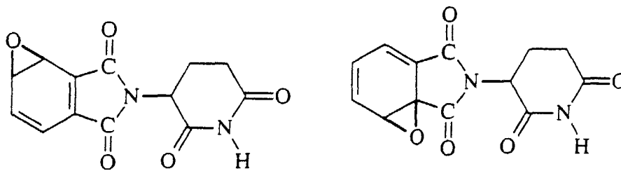
Epoxides of thalidomide
