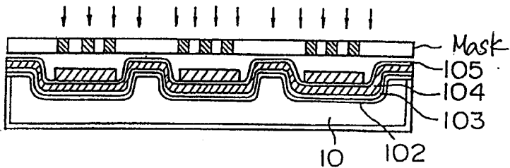
Fig. 18D Mask Exposure
