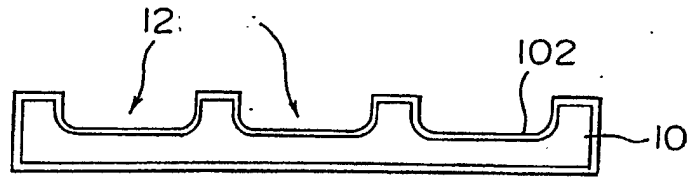
Fig. 18A Oscillating Plate Film Formation
