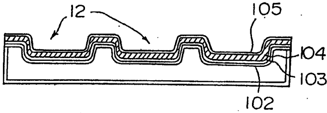
Fig. 18B Piezoelectric Substance Formation
