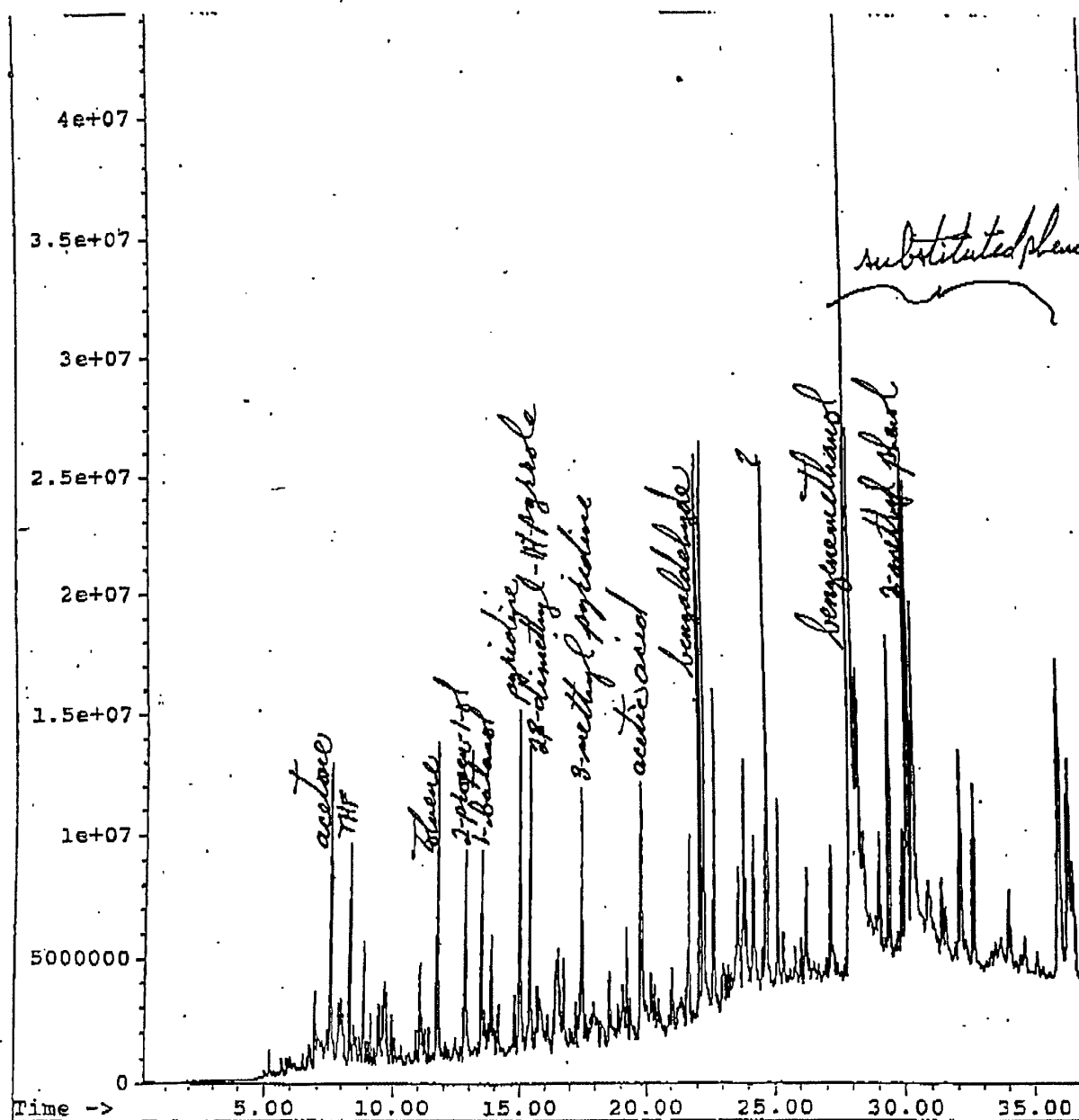
Figure 3: Pyrolysis GC/MS Chromatogram of Top Rock Material
