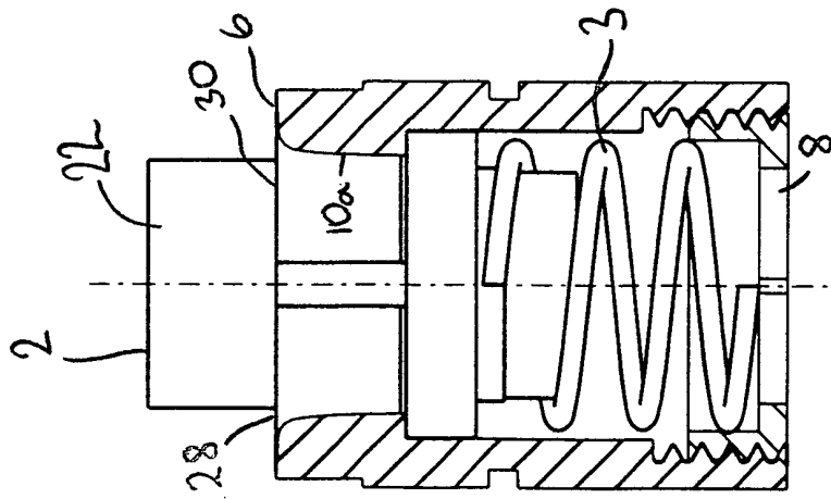
A) POSITION :- FULLY OPEN
