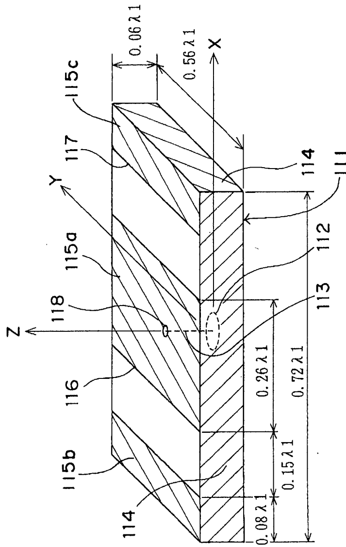
Fig.26 PRIOR ART
