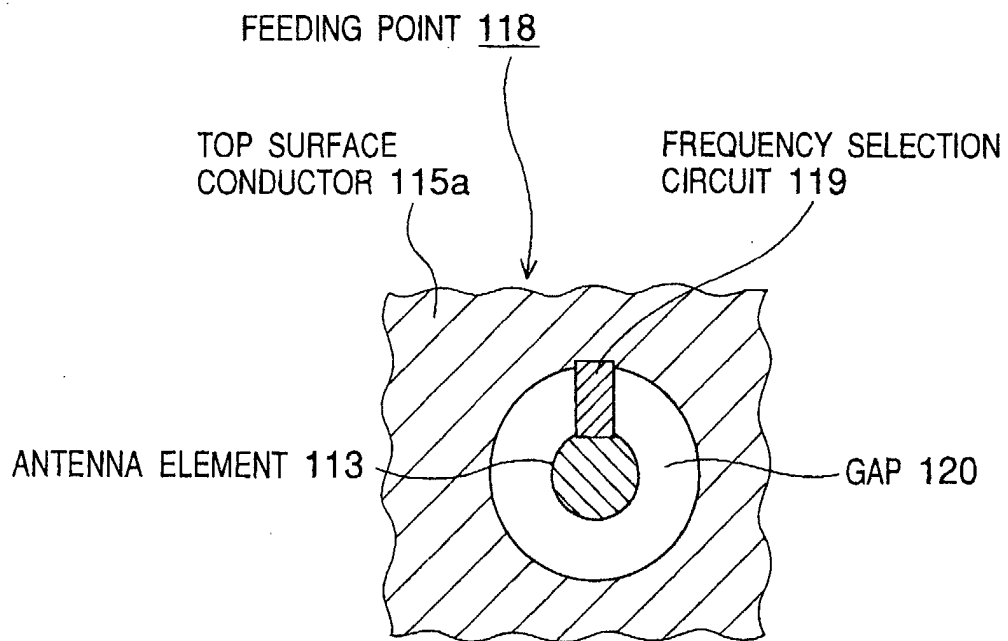
Fig.25 PRIOR ART
