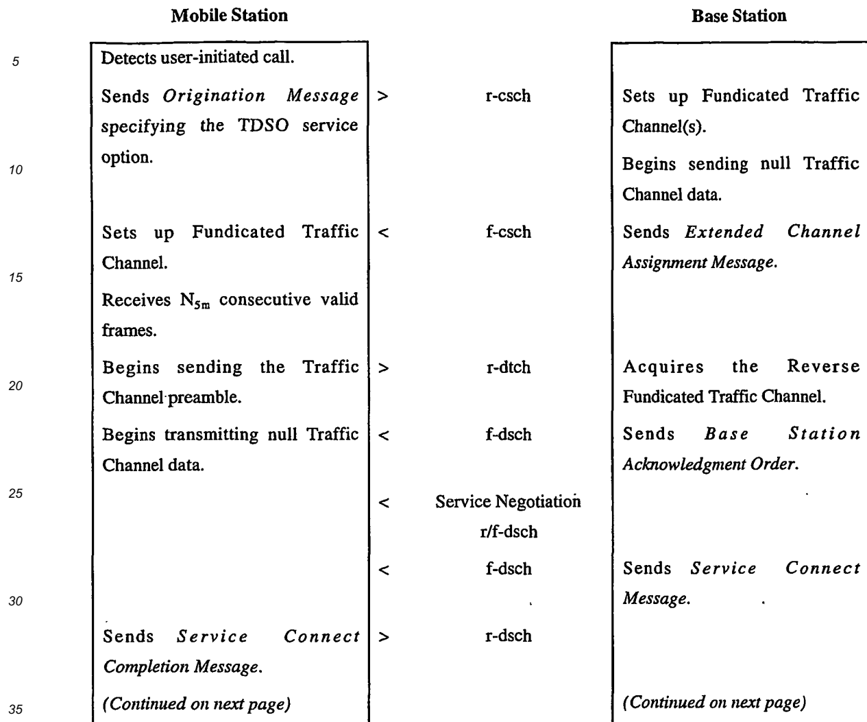
Figure 5. Mobile station origination example with transmission on DCCH/FCH/SCH (part 1 of 2)
