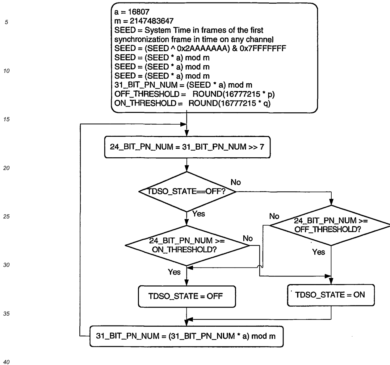
45 Figure 4. Flowchart illustrating TDSO state transitions for a D frame activity and B average "On" period in units of frames.
