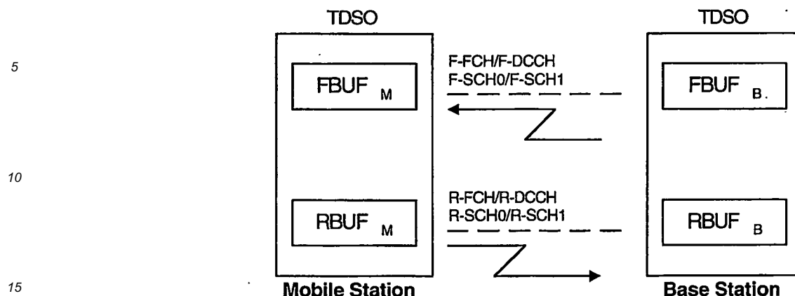
Figure 1. Synchronized operation of pseudo-random number generated buffers
