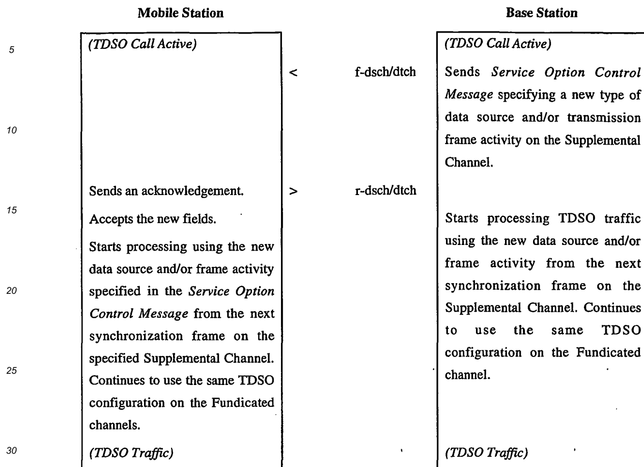
Figure 7. Base station commanded test parameters change
