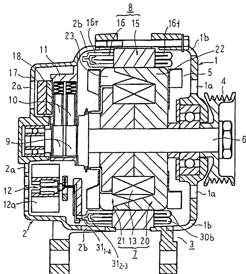
FIG. 24 PRIOR ART
