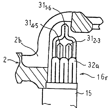
FIG. 32 PRIOR ART
