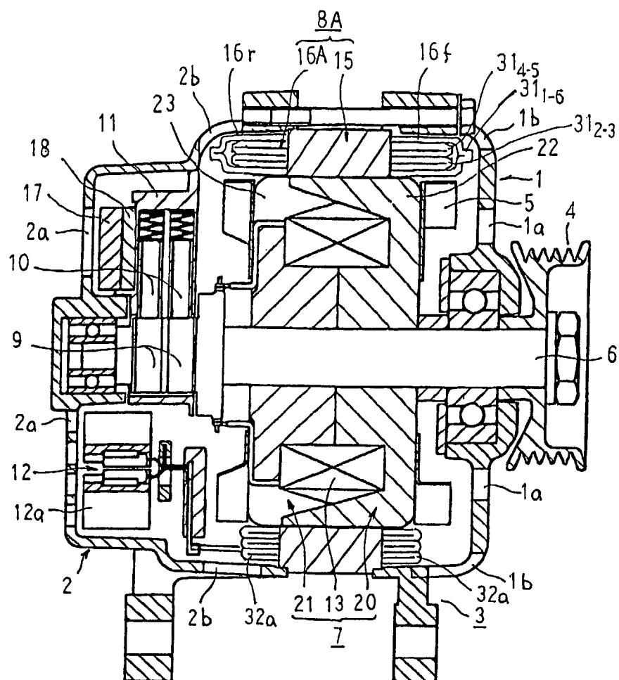
FIG. 30 PRIOR ART
