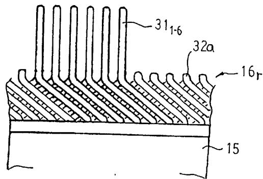
FIG. 33 PRIOR ART
