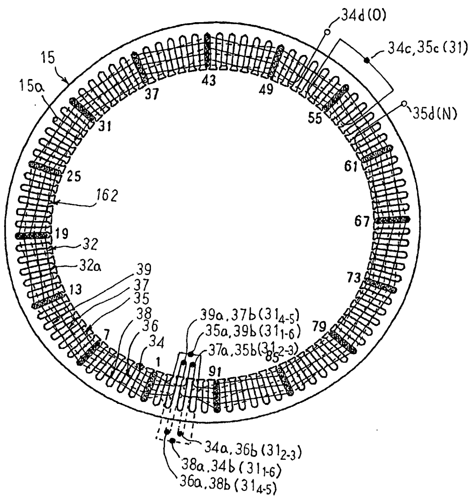
FIG. 31 PRIOR ART
