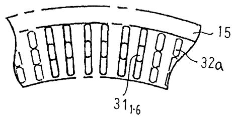
FIG. 34 PRIOR ART
