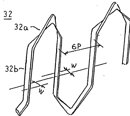
FIG. 36 PRIOR ART
