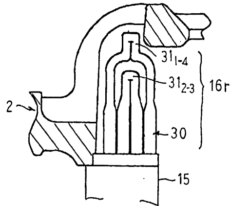
FIG. 28 PRIOR ART
