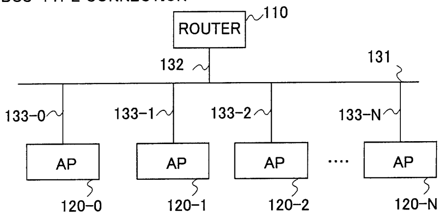
(a) BUS-TYPE CONNECTION
