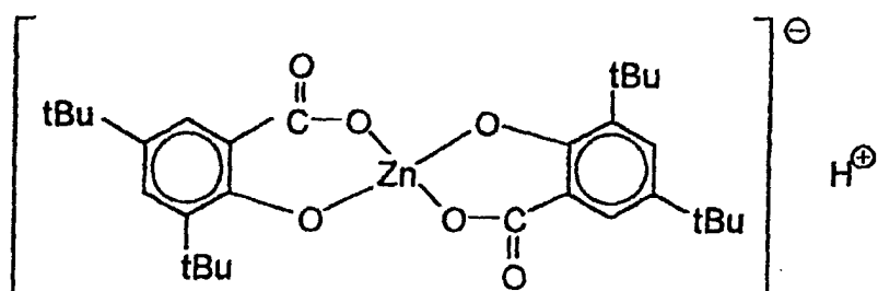
Zinc complex (10):
