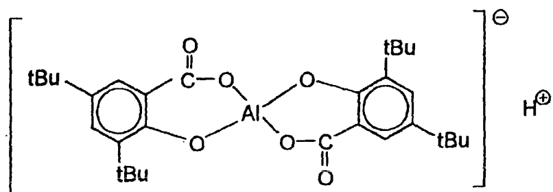
Aluminum complex (9):
