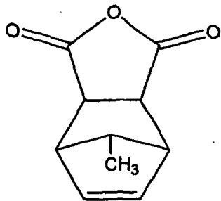
[Methylendomethylenetetrahydrophthalate anhydride]
