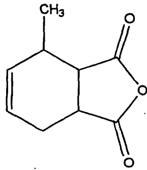
[Methyltetrahydrophthalic anhydride]
