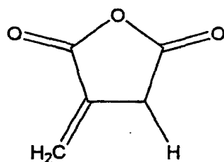
[Itaconic anhydride]
