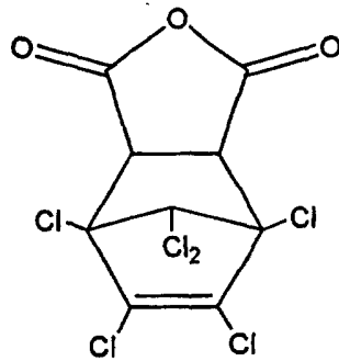
[Chlorendic anhydride]
