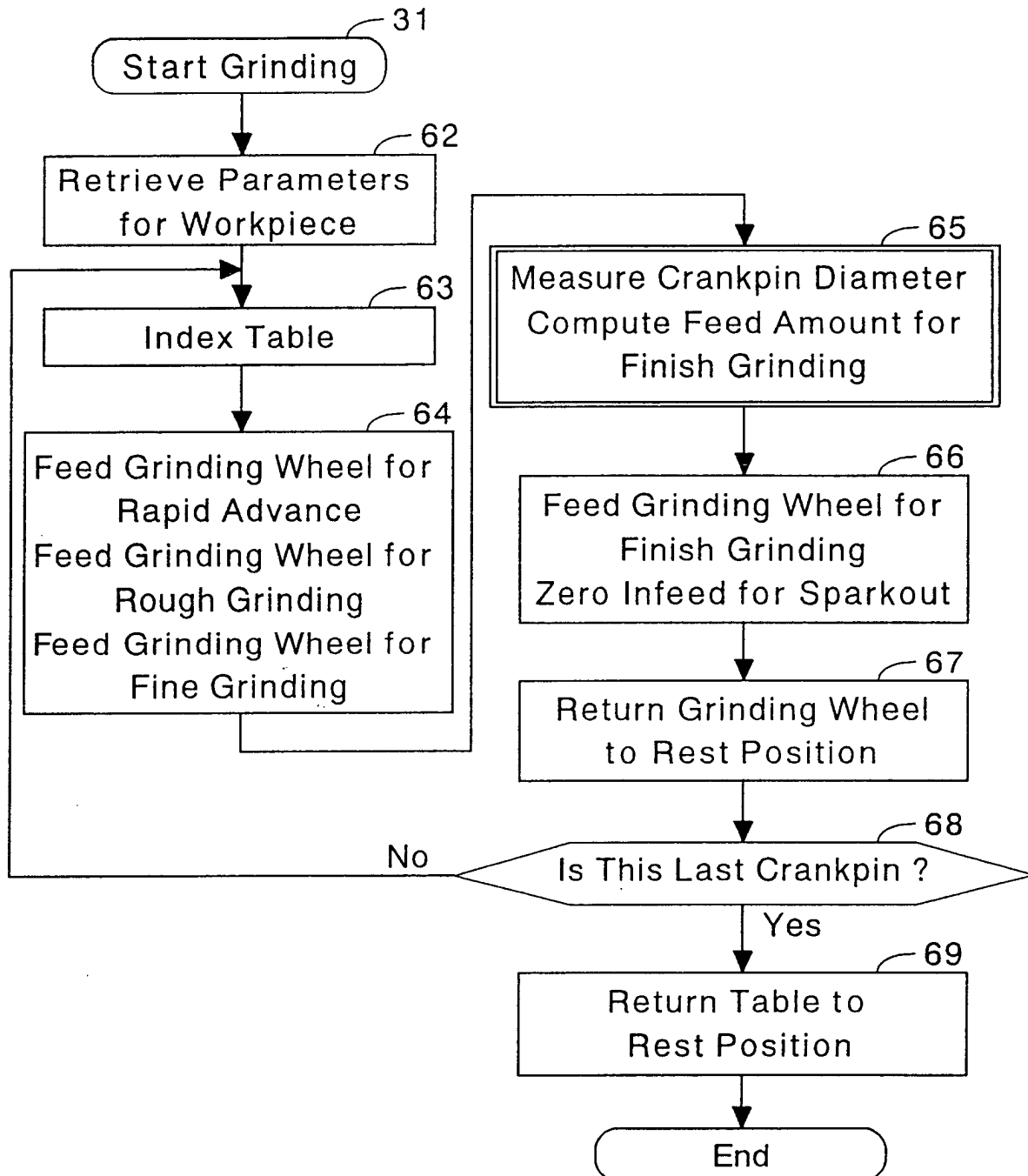
Fig.4 Program for Machining Operation
