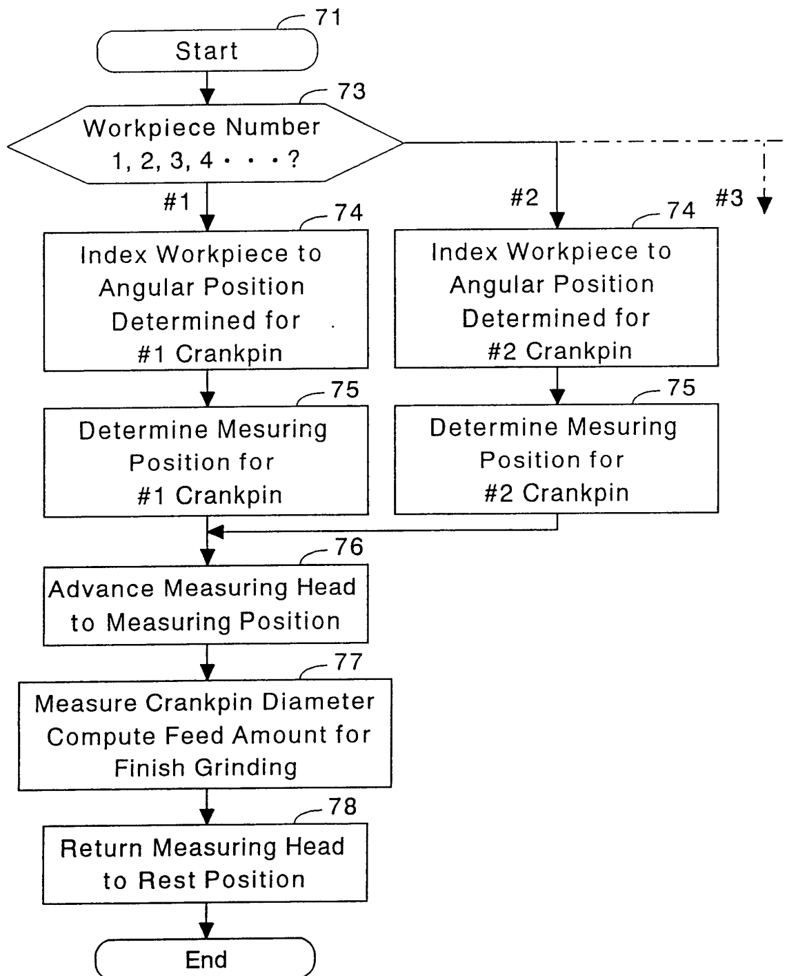
Fig.5 Program for Crankpin Diameter Measurement and Feed Amount Computation for Finish Grinding
