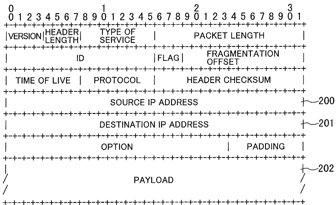
IPv4 packet format
