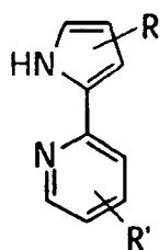
pyridylpyroles
