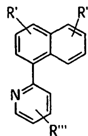
pyridynaphthalenes
