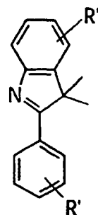
phenylindoles
