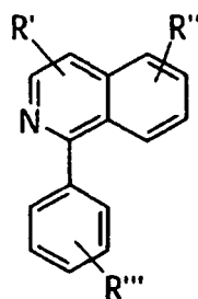
arylquinolines
