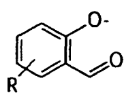
salicylaldehydes
