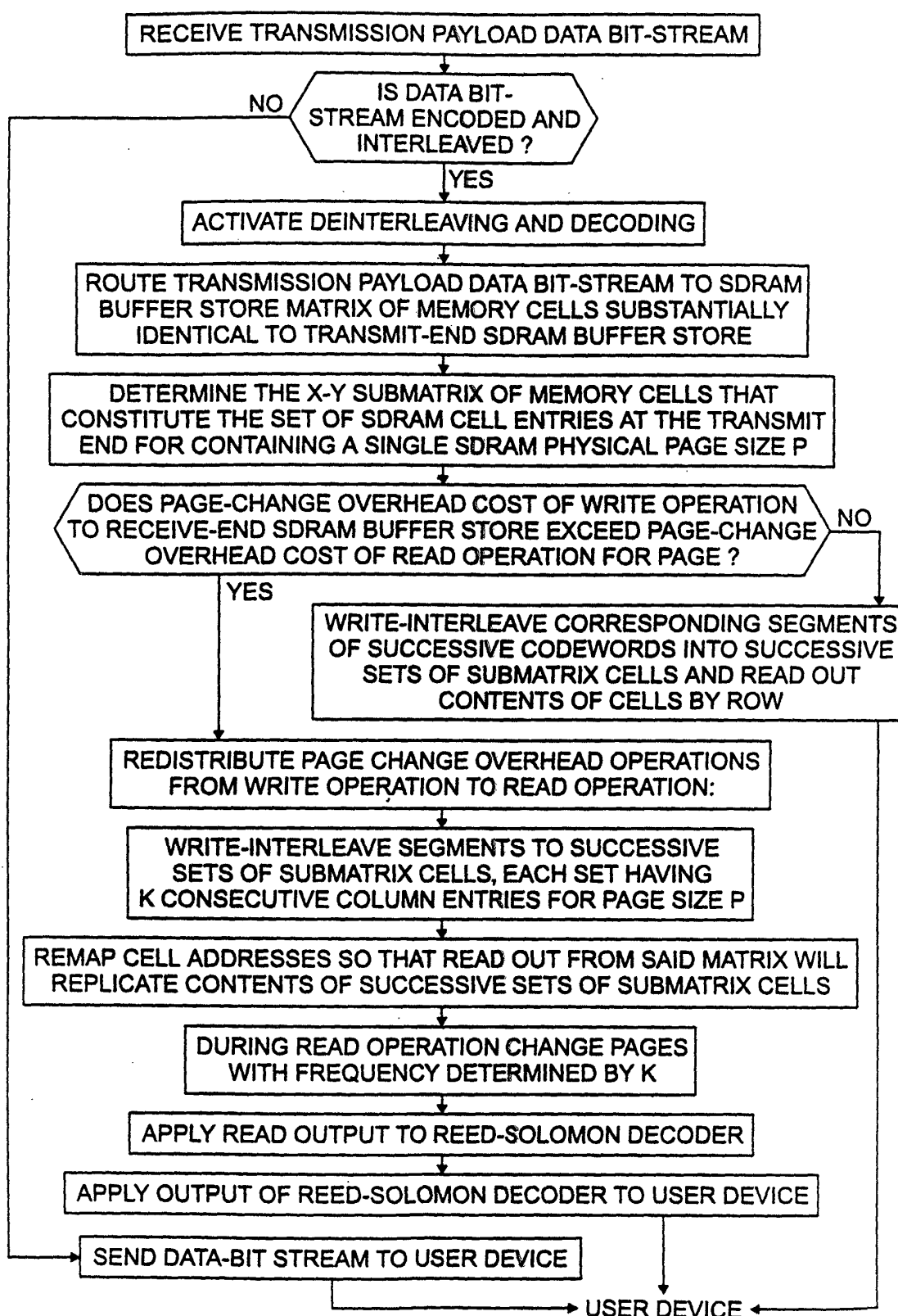
FLOW CHART OF PROCESS AT RECEIVER END
