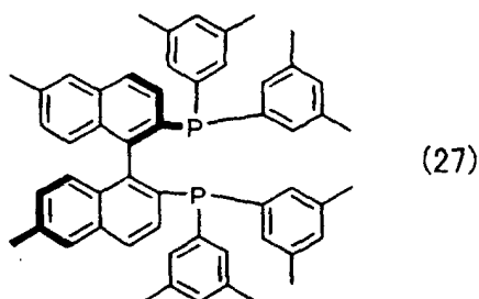
(R)-Xyl-6MeBINAP intermediate 13
