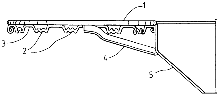
FIG. 6 PRIOR ART
