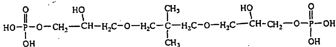
(Structure II)
