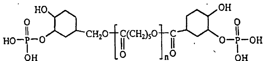
(Structure I)
