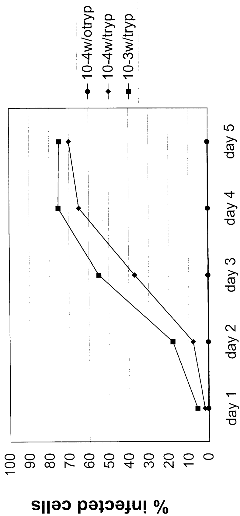
Figure 4A A/Beijing/262/95
