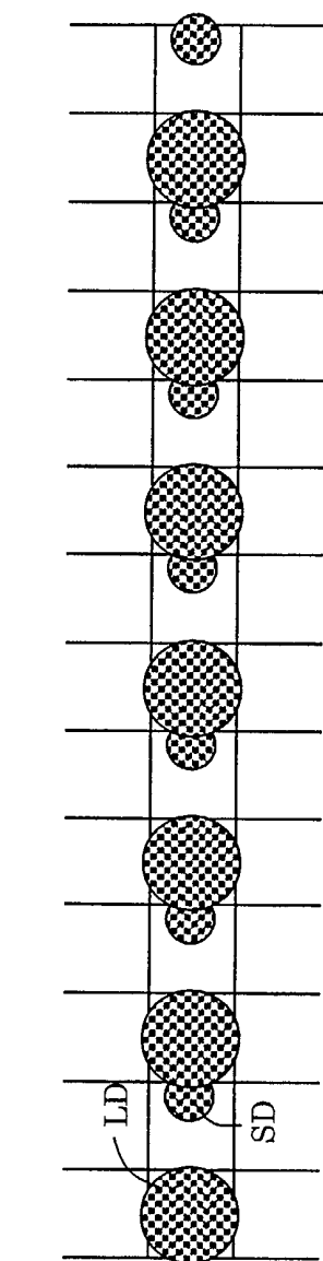
Fig. 16(A) LARGE DOT/SMALL DOT PLACEMENT MISALIGNMENT
