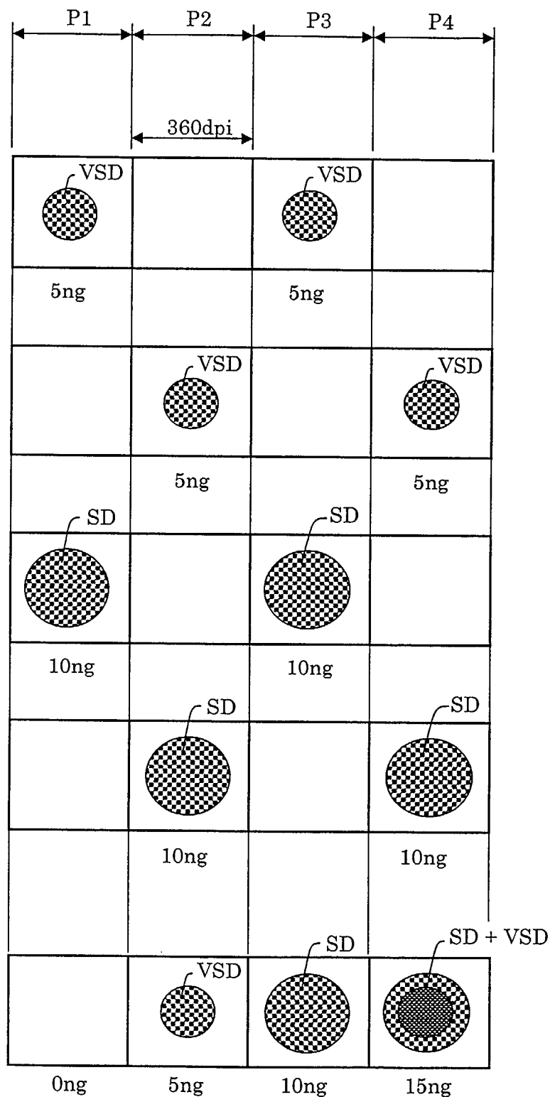
Fig. 11(E) TONE LEVELS REPRODUCIBLE WITH A SINGLE PIXEL
