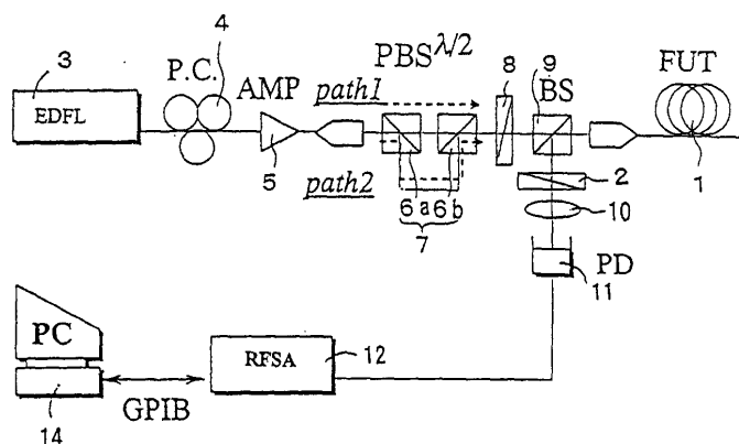
PMD MEASUREMENT SYSTEM USING FSF LASER
