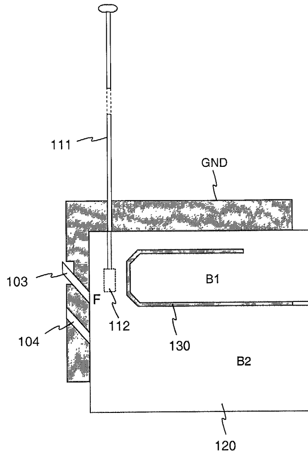
Fig. 1 PRIOR ART
