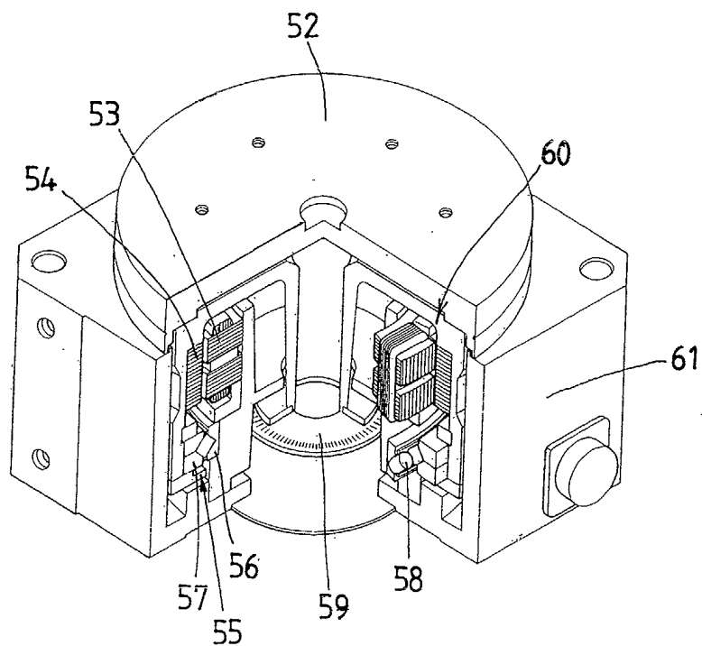
FIG. 8 (PRIOR ART)
