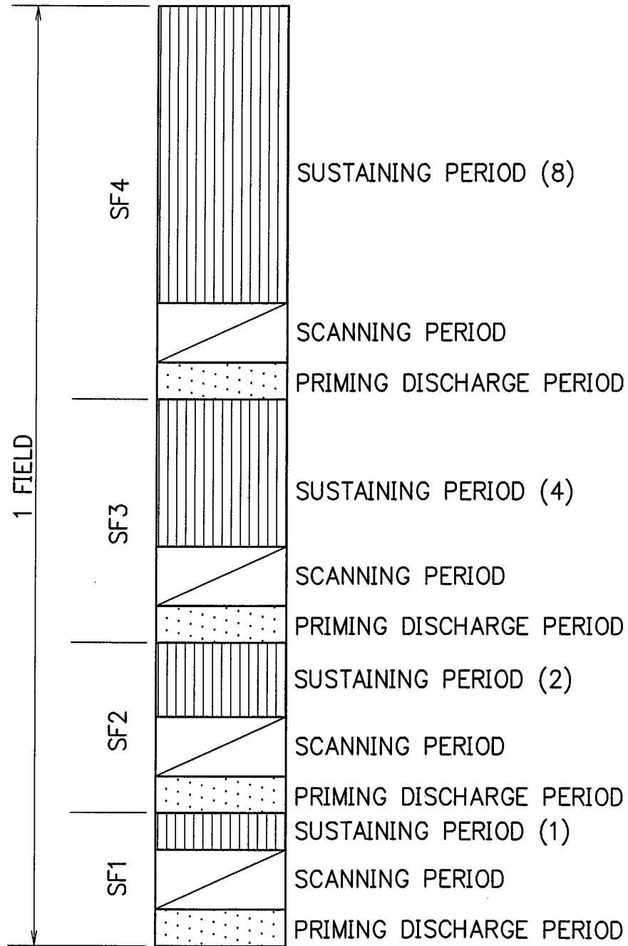
FIG. 3 PRIOR ART
