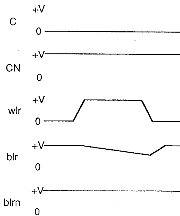
(c) Read a "zero"
