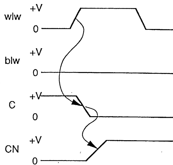
(a) Write a "zero"
