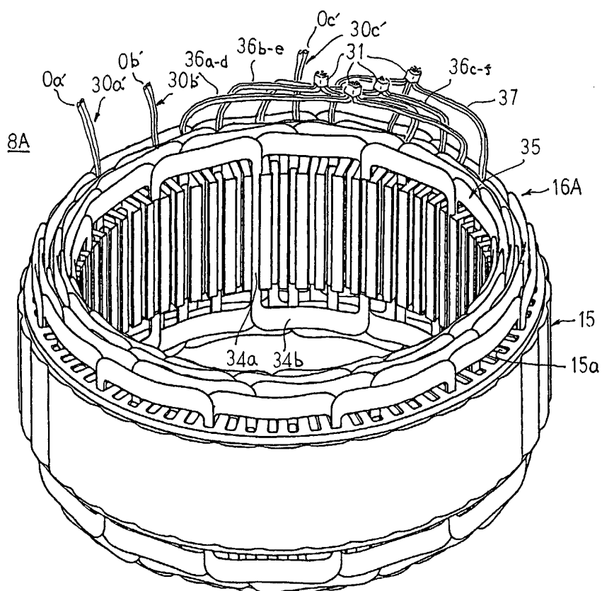
FIG. 31 PRIOR ART
