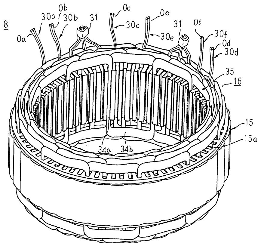
FIG. 25 PRIOR ART
