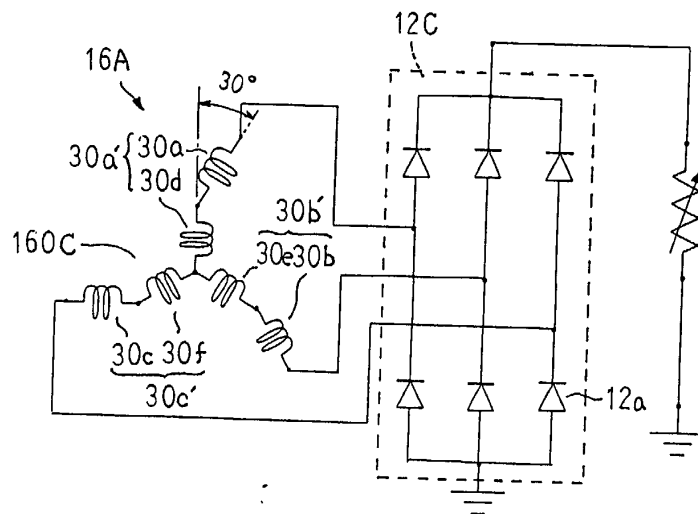
FIG. 29 PRIOR ART
