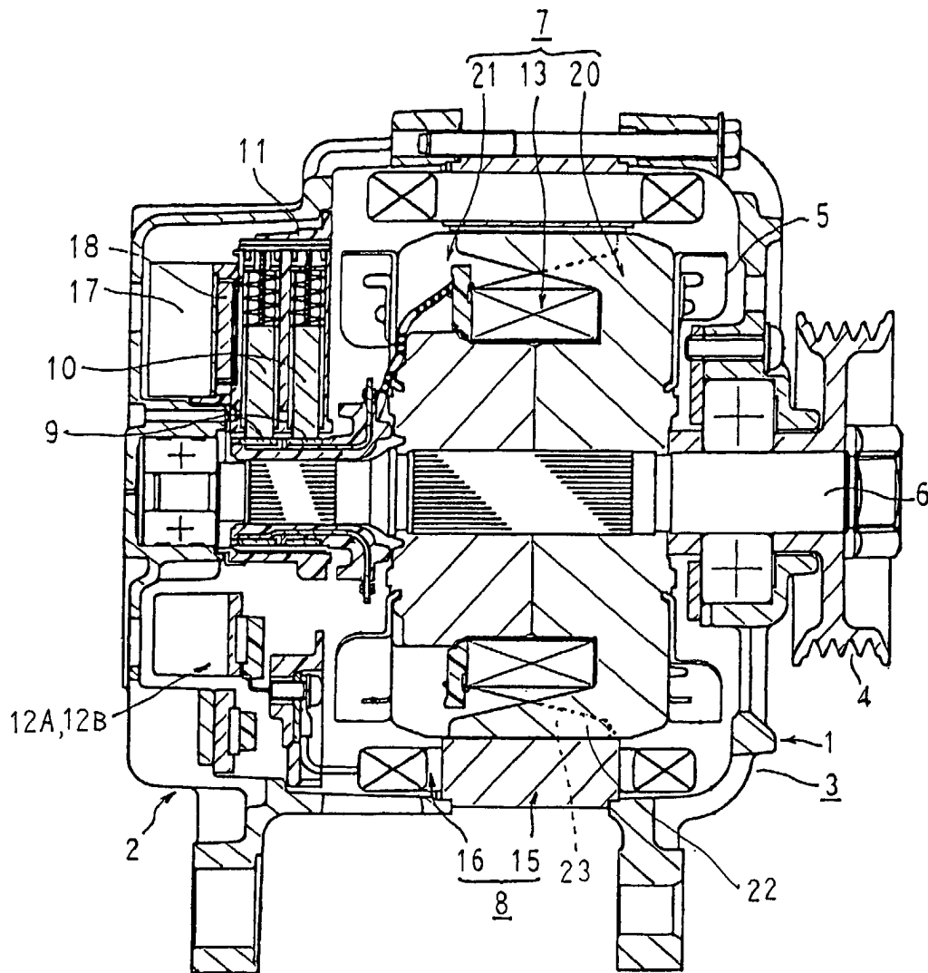
FIG. 24 PRIOR ART
