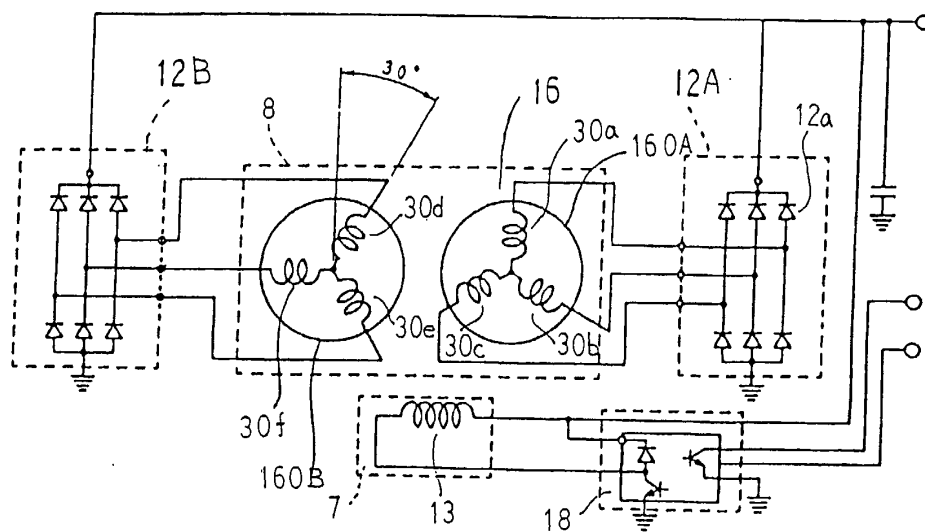
FIG. 26 PRIOR ART
