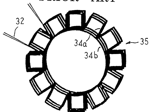
FIG. 27C PRIOR ART
