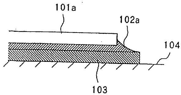
Fig. 2C (Prior Art)
