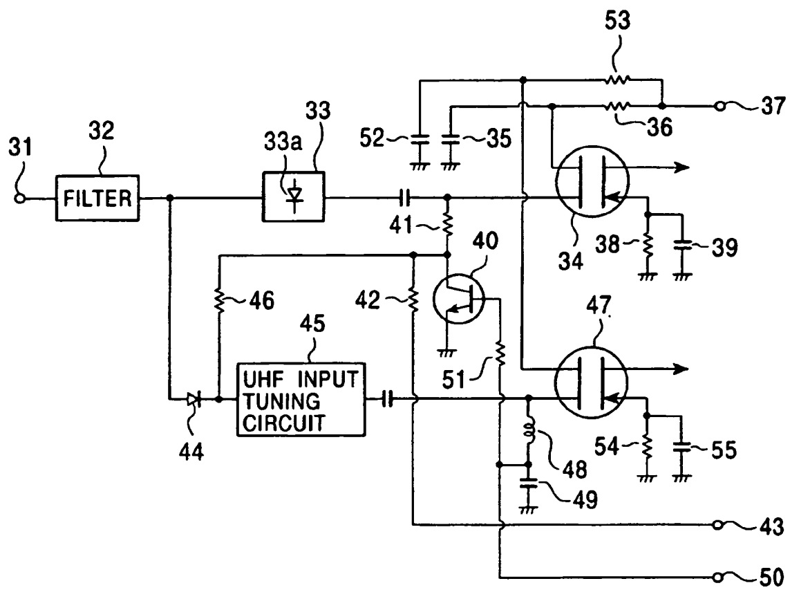
FIG. 4 PRIOR ART
