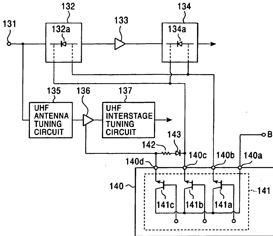
FIG. 5 PRIOR ART
