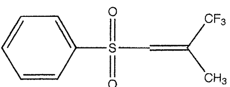
2-trifluoromethyl-2-methyl-phenyl-3- vinylsulphone or phenyl trifluoroisobutenyl sulphone
