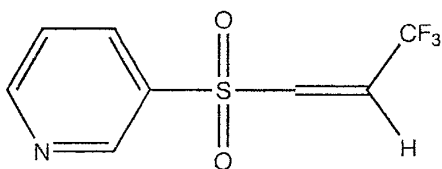
3,3,3-trifluoro-1-(pyridylsulphonyl)-1-propene or pyridyl trifluoropropenyl sulphone
