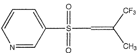
2-trifluoromethyl-2-methyl-pyridine-3- vinylsulphone or pyridyl trifluoroisobutenyl sulphone
