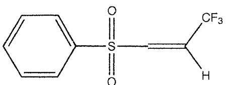
3,3,3-trifluoro-1-(phenylsulphonyl)-1-propene or phenyl trifluoropropenyl sulphone
