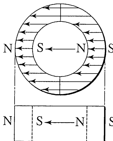
PARALLEL MAGNETIZATION
