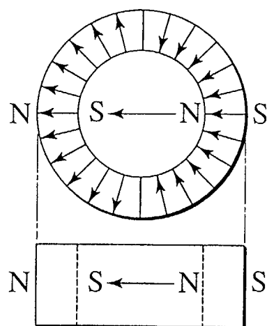
RADIAL MAGNETIZATION
