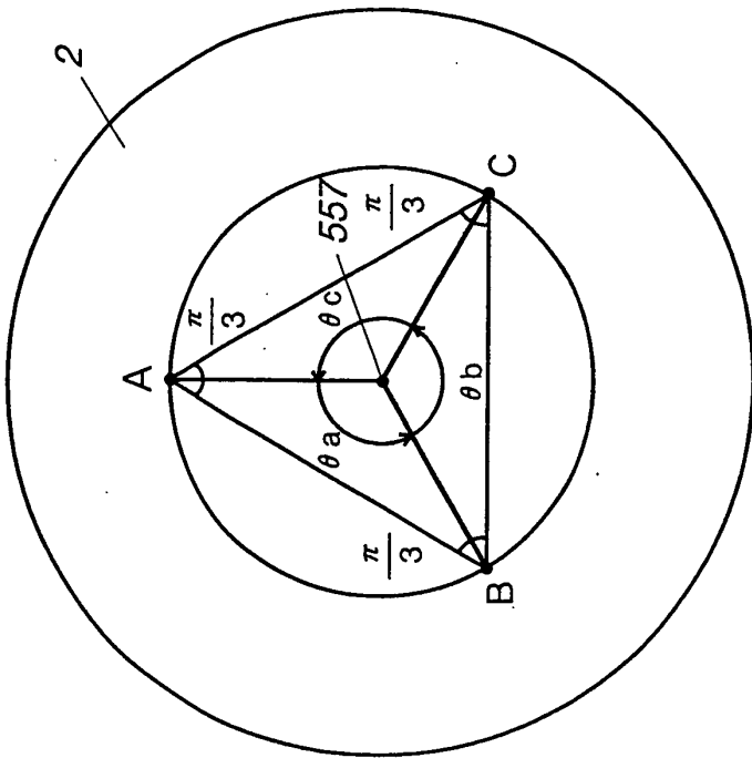
FIG. 19A IN THE CASE OF NO ECCENTRICITY
