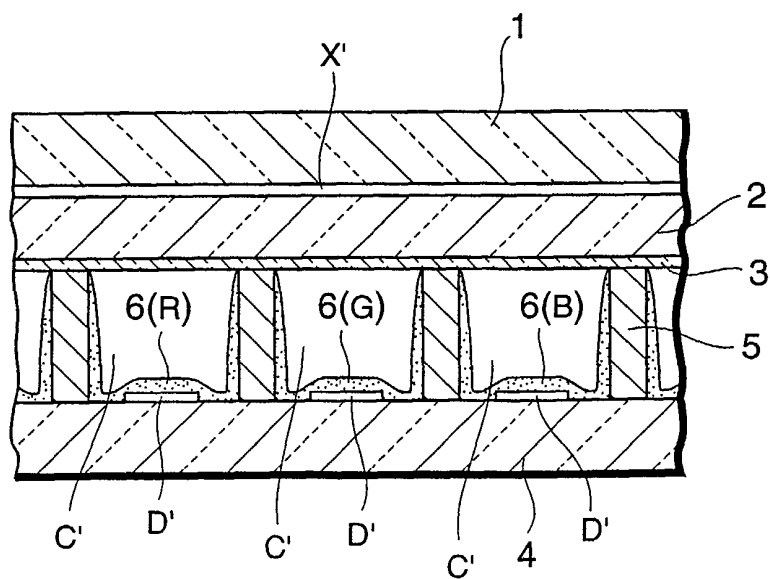
FIG.12 PRIOR ART SECTION W-W
