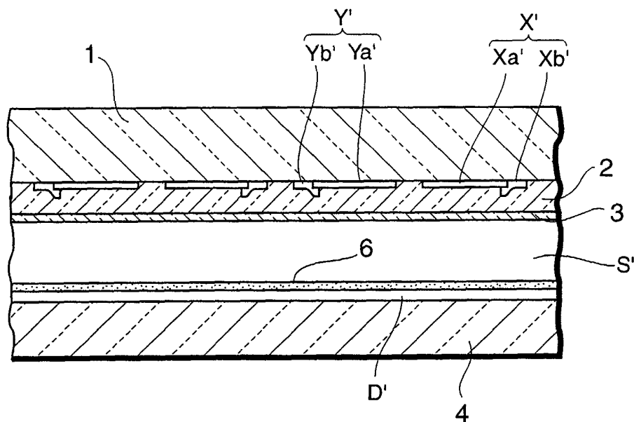
FIG.11 PRIOR ART SECTION V-V
