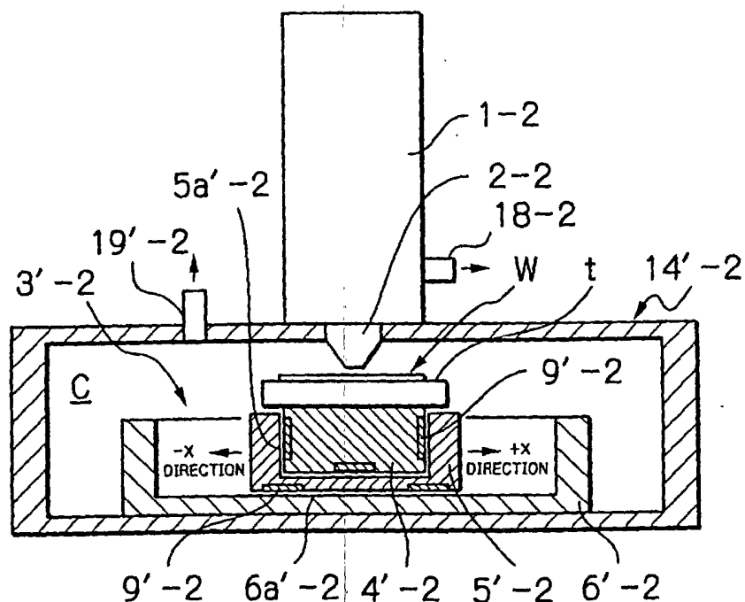
Fig.17(B) PRIOR ART
