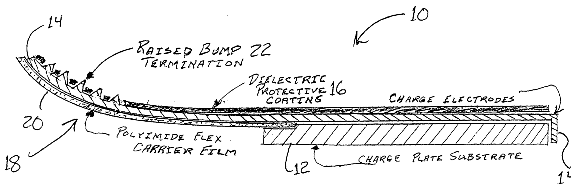
FIG. 1. INTEGRATED CHARGE PLATE/FLEXIBLE CABLE ASSEMBLY
