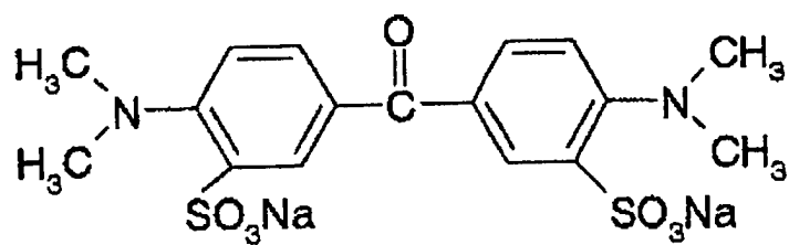
Yellow Dye Compound-1
