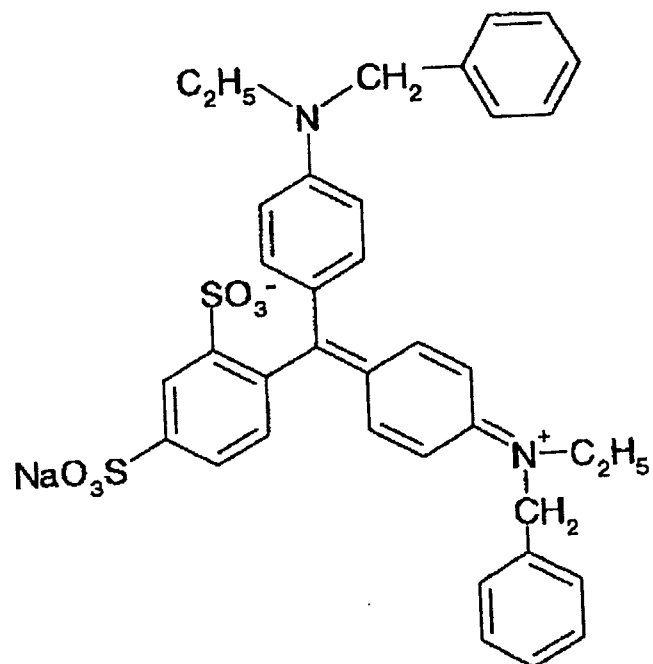
Blue Dye Compound-1
