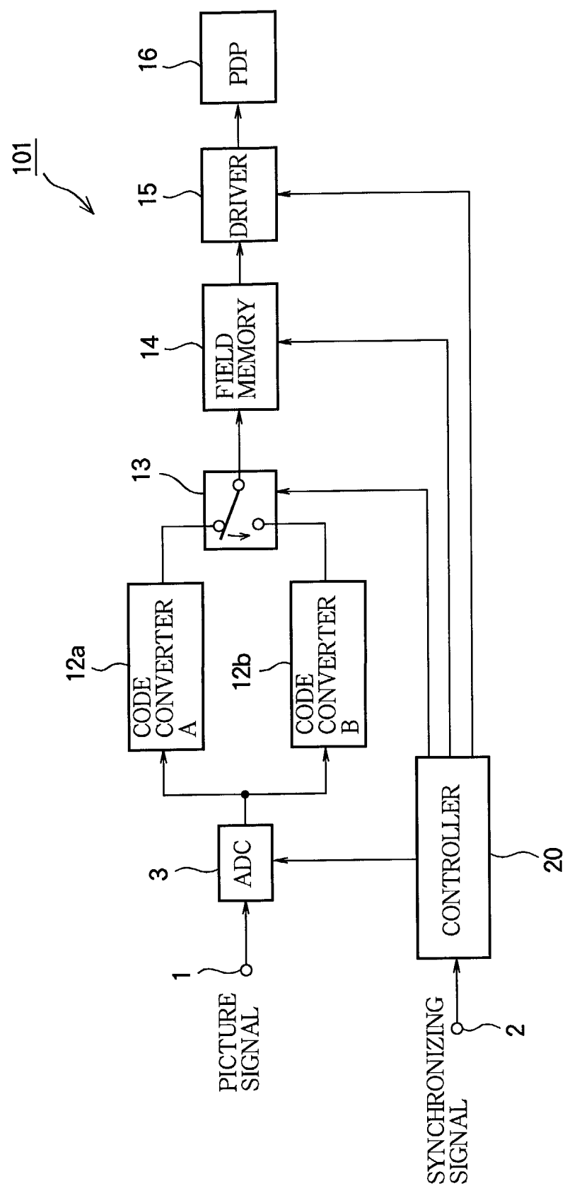
FIG. 21 PRIOR ART
