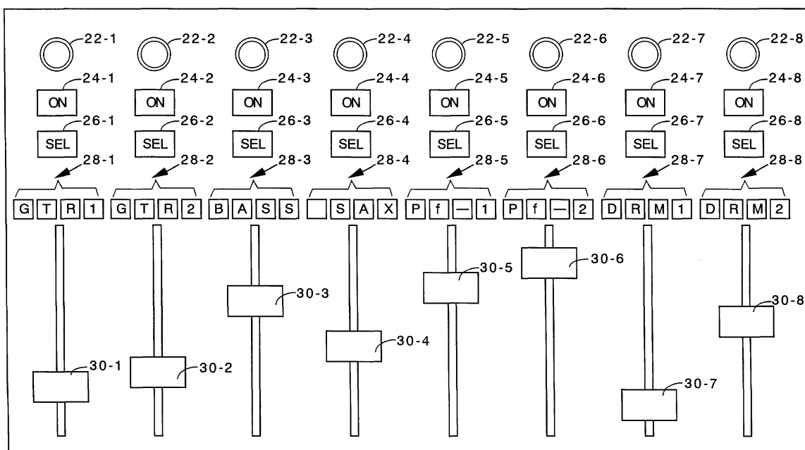
Fig. 6 Control Panel
