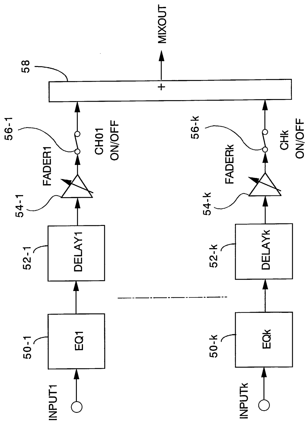
Fig.2 DSP Algorithm
