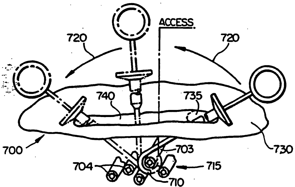
FIG. 113 (PRIOR ART)
