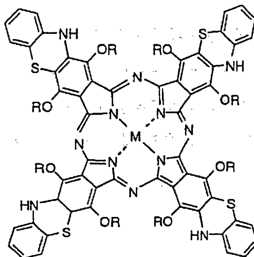
(IR-27) M=VO, R=i-C 5 H 11
