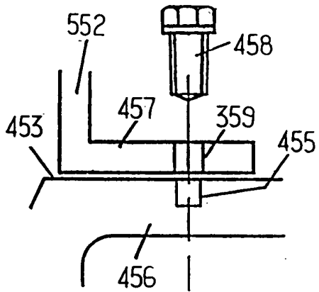
FIG. 11C (PRIOR ART)
