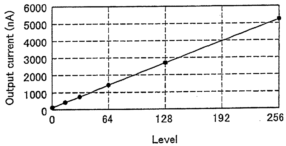
Output Current Characteristics
