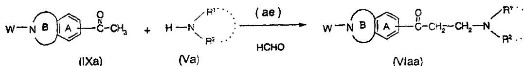
[Reaction scheme 1-2]
