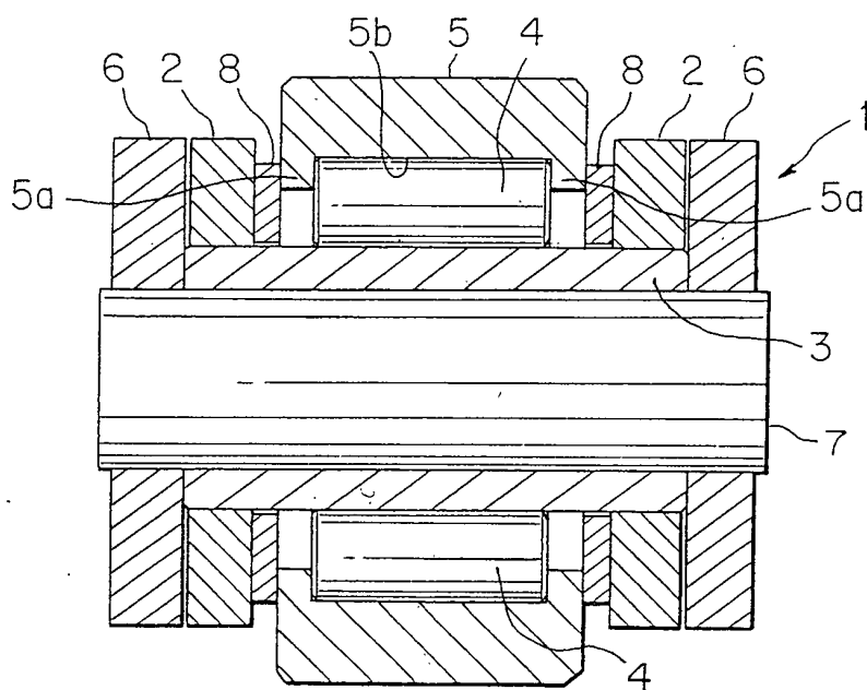
FIG. 18 PRIOR ART
