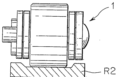
FIG. 19 PRIOR ART
