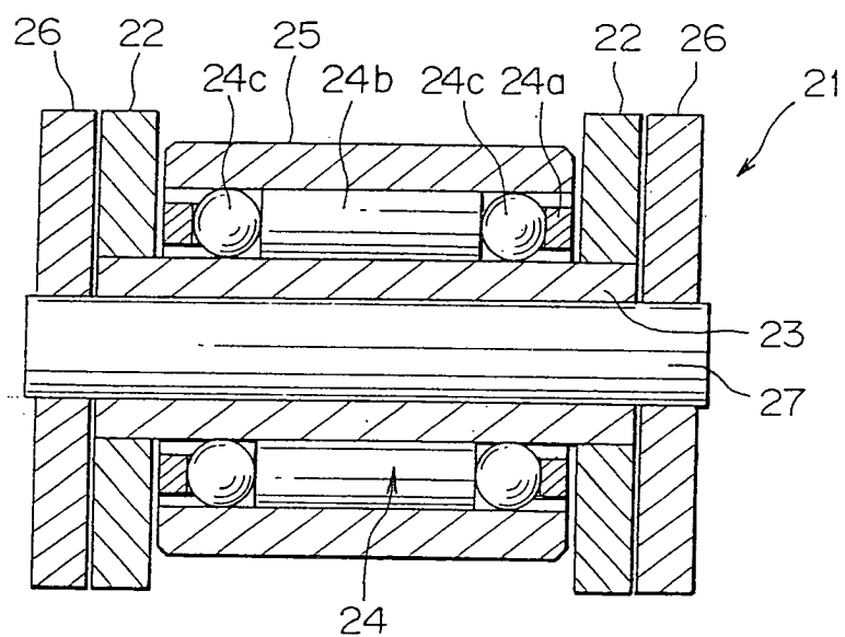
FIG. 22 PRIOR ART
