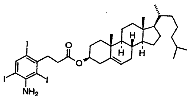
Compound (2)
