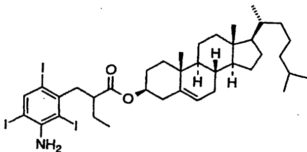
Compound (3)
