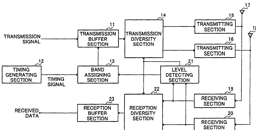
BASE STATION 10
