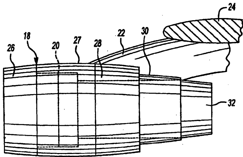
Fig-1 PRIOR ART
