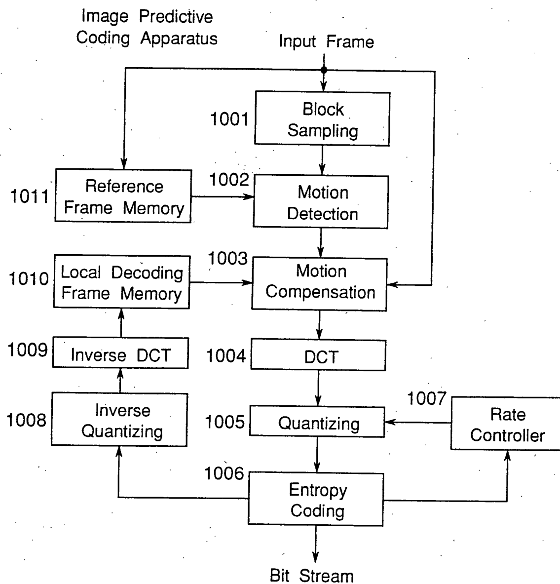
Fig.14 PRIOR ART
