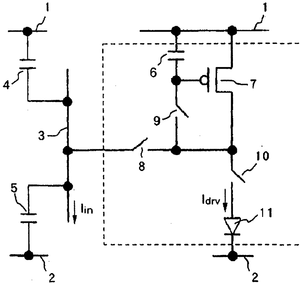
FIG. 1 (BACKGROUND ART)
