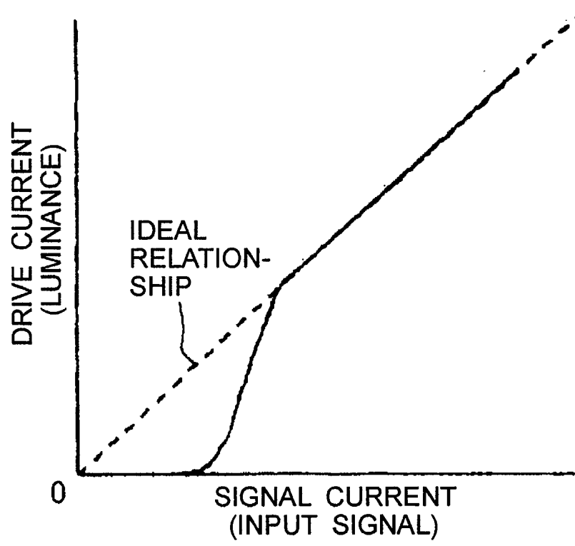
FIG. 3 (BACKGROUND ART)
